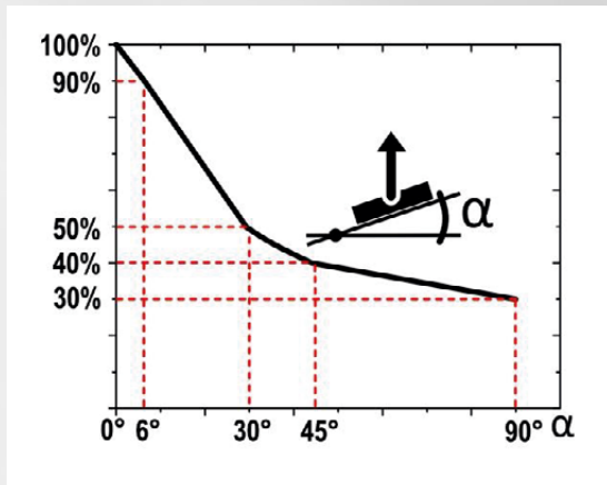
Load-figures corresponding to the direction for the TML 90 R
